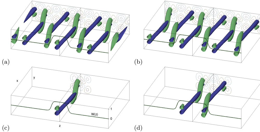
FIGURE 2. Construction of localized initial guesses by windowing. (a,b) The spatially periodic EQ7 solution of plane Couette flow, in two spatial phases. Three copies of the \alpha, \gamma = 1, 2 periodic solution at Re = 400 are shown in the z \in [-3\pi/2, 3\pi/2] subset of the full L_x, L_z = 2\pi, 6\pi computational domain, with the z = 0 plane shown bisecting the box to highlight the z symmetries. The solutions in (a) and (b) are related by a quarter-wavelength phase shift in z . (c,d) Initial guesses for localized solutions with different symmetry groups, produced by multiplying (a,b) by windowing functions W(z) (heavy line in front planes). Isosurfaces of signed swirling strength at s = \pm 0.12 are shown in (green/blue) and contours of streamwise velocity in the back plane at contour levels u = \pm 0.03 \cdot [1:2:9] .
