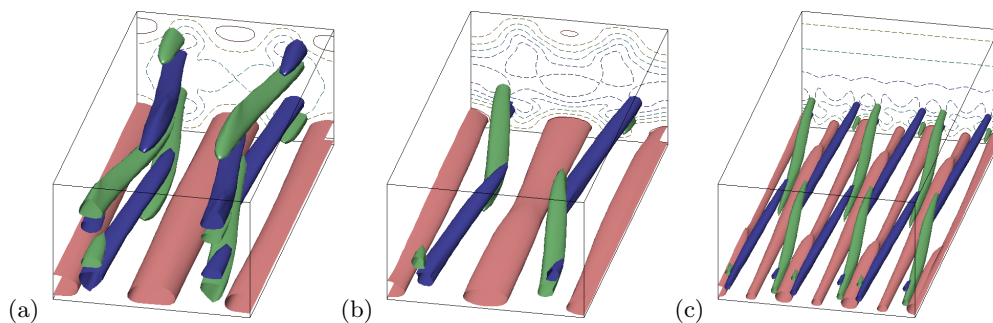
FIGURE 6. Spatially periodic traveling waves of channel flow with decreasing wall-normal symmetry. (a) TW1, constructed by continuing EQ7 from plane Couette to channel conditions, has symmetry group \langle \sigma_y, \sigma_z, \tau_{xz} \rangle . Isosurfaces of signed swirling strength at s = \pm 0.04 are shown in green/blue. High-speed streaks near the lower wall are shown by isosurfaces of streamwise velocity at u = 0.02 . High-speed streaks near the upper wall, symmetric to those near the lower wall, are not shown as isosurfaces but they are indicated in the contour plots of streamwise velocity in the back plane. (b) TW2, found from an initial guess judiciously chosen from numerical simulation data, has symmetry group \langle \sigma_z, \tau_{xz} \rangle . Isosurfaces of signed swirling strength at s = \pm 0.10 are shown in green/blue, and high-speed streaks near the lower wall are shown by isosurfaces of streamwise velocity at u = 0.03 . There are similar but weaker vortex structures and high-speed streaks near the upper wall, but they do not appear at these levels for the isosurfaces. Both (a) and (b) are shown at \alpha, \gamma = 1, 2 and Re = 2300 . (c) TW3, constructed by continuation in Reynolds number from TW2 and further symmetrization and Newton-Krylov refinement, has \langle \sigma_z, \tau_{xz} \rangle but periodicity \alpha, \gamma = 1, 6 , and is shown at Re = 4000 . Isosurfaces of signed swirling strength are at s = \pm 0.9 and u = 0.03 . Each back plane shows contour plot of streamwise velocity at levels u = \{0.03, -0.03, -0.09, -0.15, \dots\} , positive in solid lines and negative in dashed.
